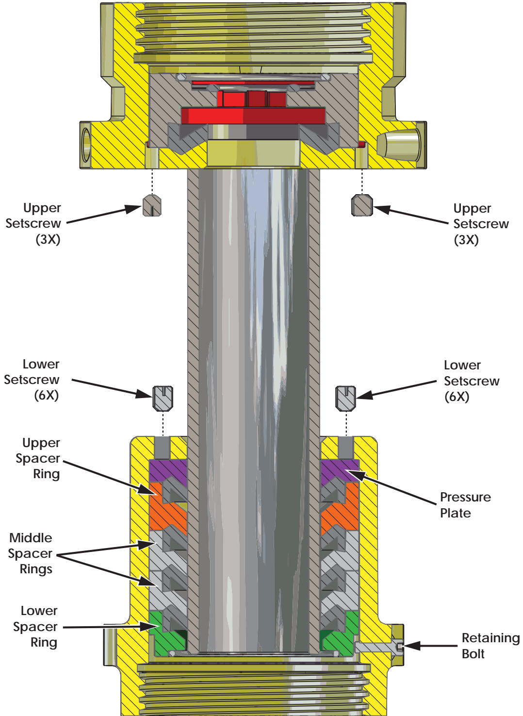
Figure 4: Washpipe Assembly Cross-section
