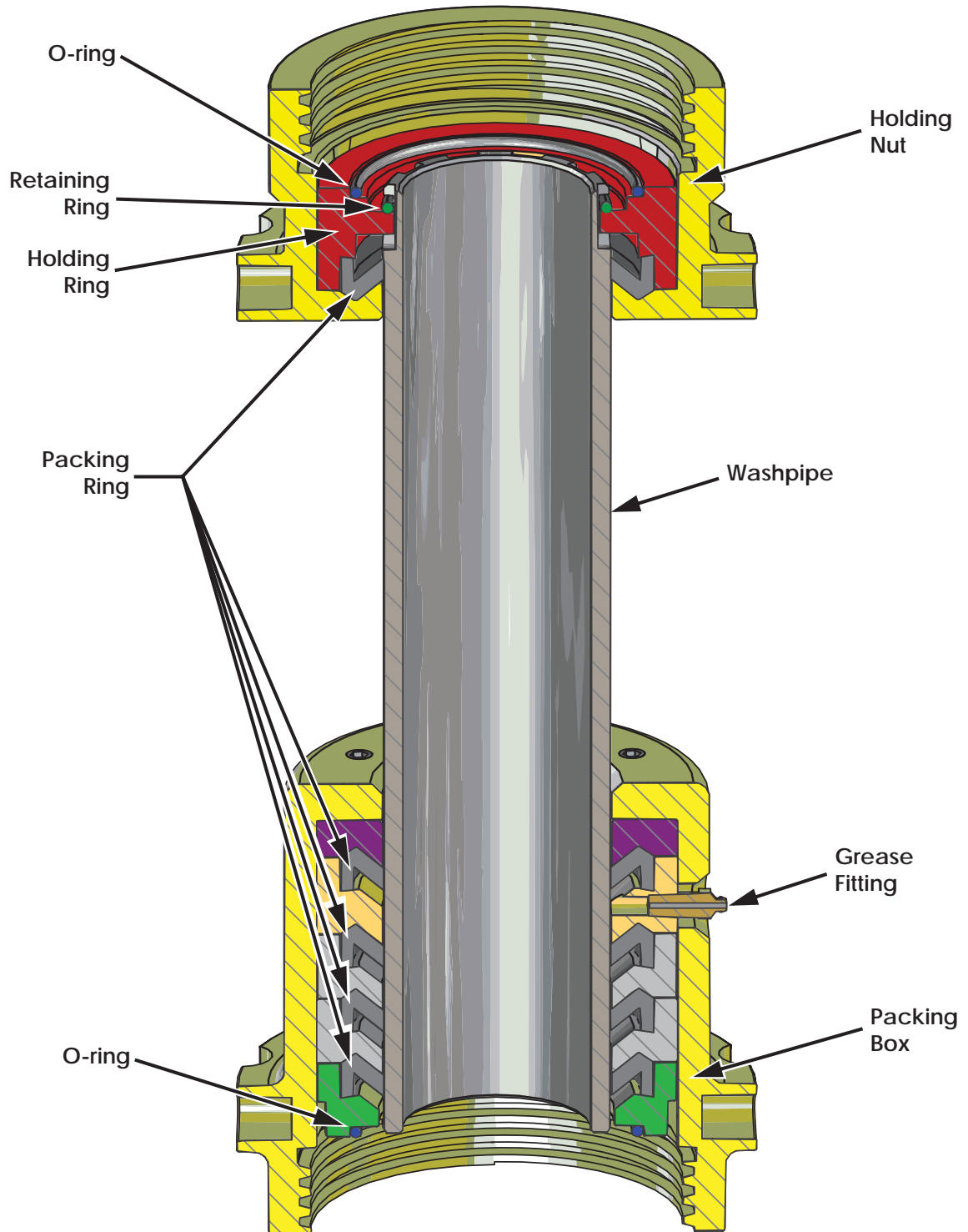
Figure 3: Washpipe Assembly Cross-section
